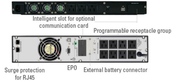
UPS Rear View VD1000A1U (top) & VD1000A (bottom)
